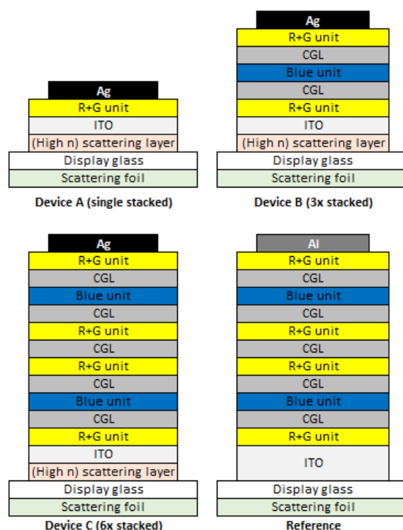
Figure 1: Device structures
