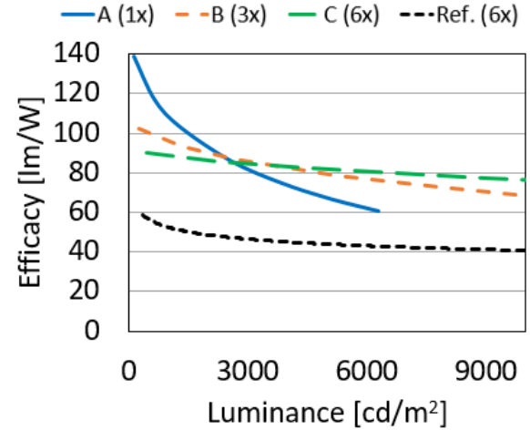
Figure 3: Luminous efficacy
